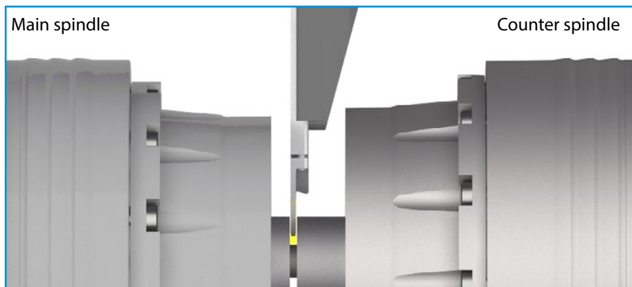
Machining in narrow spaces (for instance operations with counter spindle)
