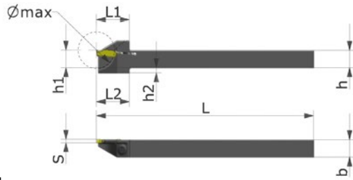
LH holder Radially reinforced
