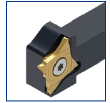
RH holders for RH inserts
