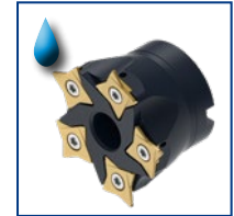
Milling head with 5 insert pockets
