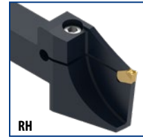
CLCBL..X Standard Design
