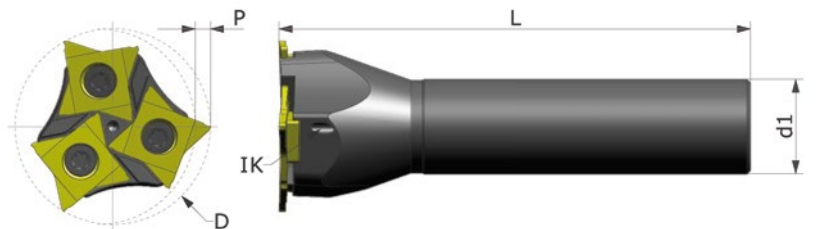
Shank end mill with more than one insert pocket
